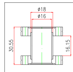
Standard nipple CF16
